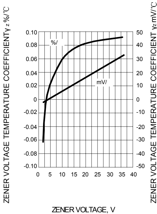
FIG.2 – TEMPERATURE COEFFICIENT
