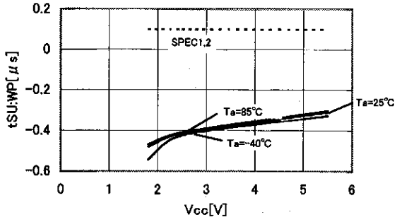
WP SETUP TIME t_{SU:WP}
