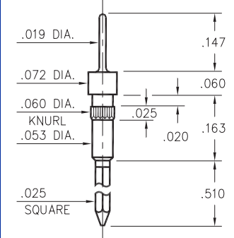
5301-0-05-XX-00-00-01-0 Press-fit in .057 mounting hole
