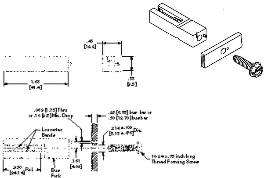
Part Number 194257-1
