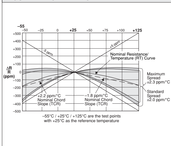
FIGURE 1 - NOMINAL TCR
