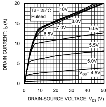
Fig.2 Typical Output Characteristics(I)
