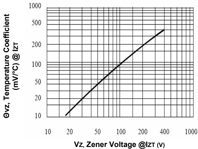
Fig.3-Typical Temperature Coefficients
