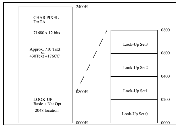
Fig.24 ROM Organisation
