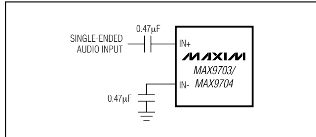
Figure 3. Single-Ended Input
