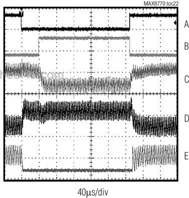
PSI + 1-LSB TRANSITION
