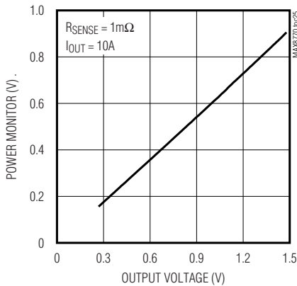
POWER MONITOR vs. OUTPUT VOLTAGE
