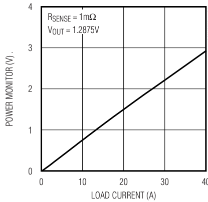
POWER MONITOR vs. LOAD CURRENT
