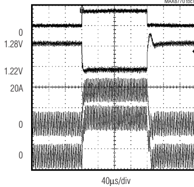
HFM LOAD TRANSIENT ( V_{OUT(HFM)} = 1.2875V )
