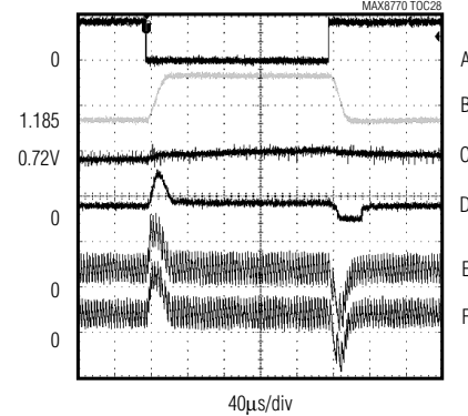
POWER MONITOR - VID TRANSITION RESPONSE
