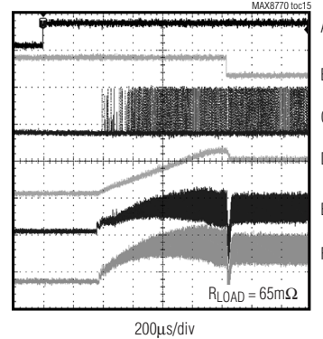
SOFT-START (UP TO CLKEN)
