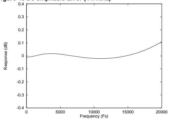
Figure 48 De-emphasis Error (48kHz)
