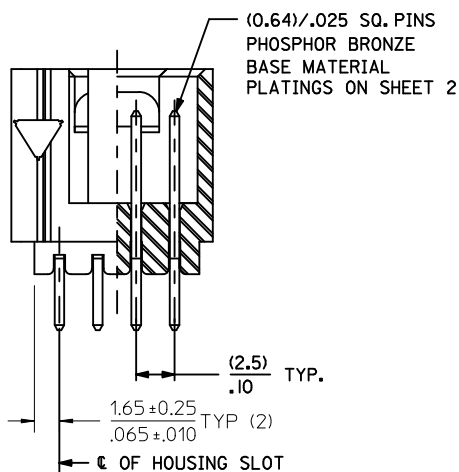
SECTION E-E
