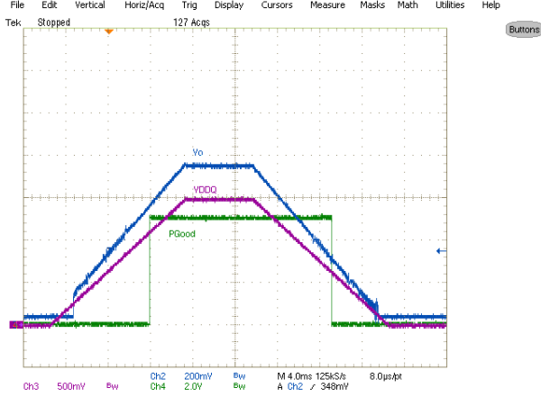
Fig. 14: Tracking -3A load, sinking current, Ch2:V out , Ch3: I L , Ch4:V DDQ , Ch5:PGood
