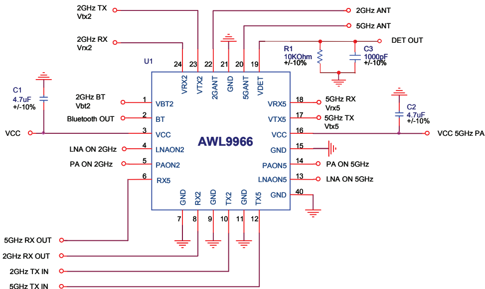
Figure 12: Application Circuit
