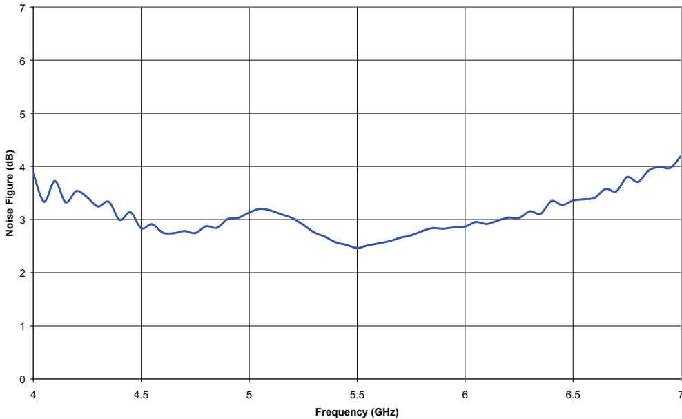
Figure 10: 5 GHz Band Noise Figure vs Frequency (T c = +25 °C, V CC = +3.3 V, LNA ON5 = +3.3 V, V RX5 = +3.3 V, V TX5 = 0 V)
