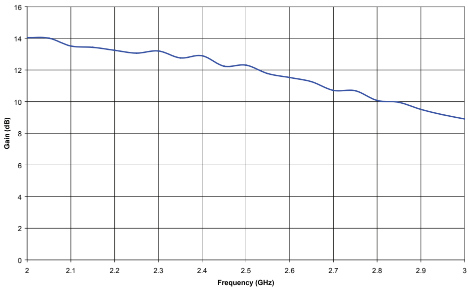
Figure 6: 2 GHz Band RX Gain vs Frequency (T c = +25 °C, V CC = +3.3 V, LNA ON2 = +3.3 V, V RX2 = +3.3 V, V TX2 = V BT2 = 0 V)
