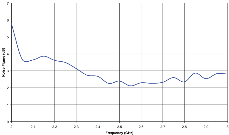
Figure 5: 2 GHz Band Noise Figure vs Frequency (T c = +25 °C, V CC = +3.3 V, LNA ON2 = +3.3 V, V RX2 = +3.3 V, V TX2 = V BT2 = 0 V)
