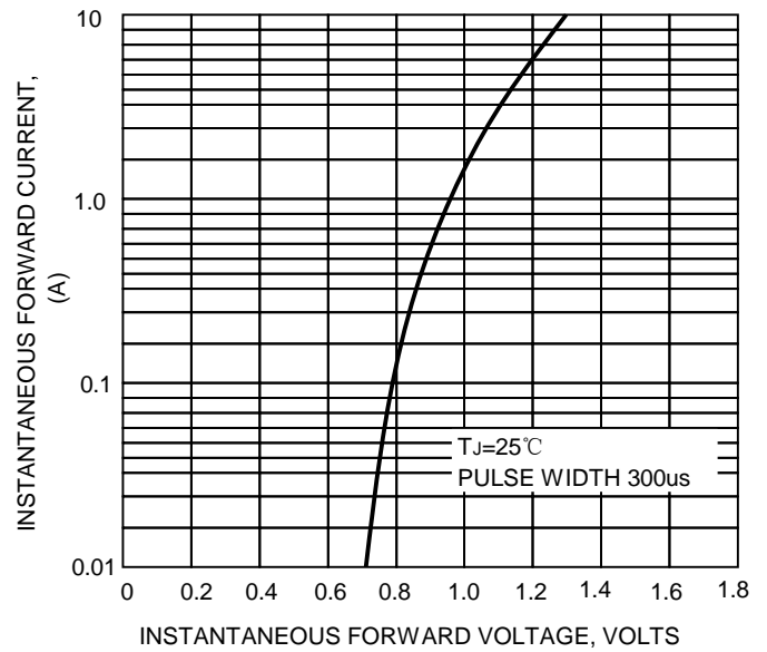
FIG.4-TYPICAL FORWARD CHARACTERISTICS
