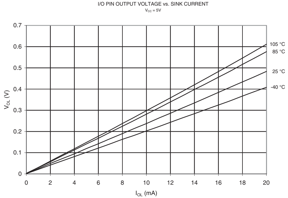
Figure 2-32. V_{OL} : I/O Pin Output Voltage vs. Sink Current ( V_{CC} = 5V )
