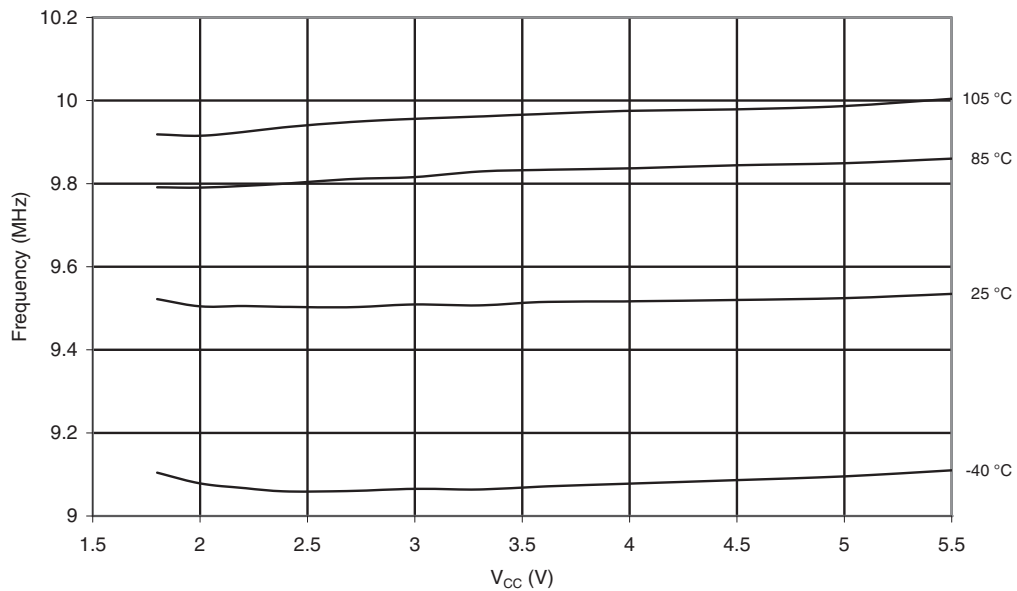
Figure 2-55. Calibrated 4.8 MHz Oscillator Frequency vs. Temperature
