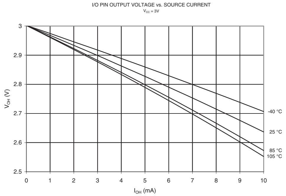
Figure 2-28. V_{OH} : I/O Pin Output Voltage vs. Source Current ( V_{CC} = 3V )
