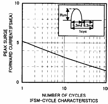
IFSM-CYCLE CHARACTERISTICS
