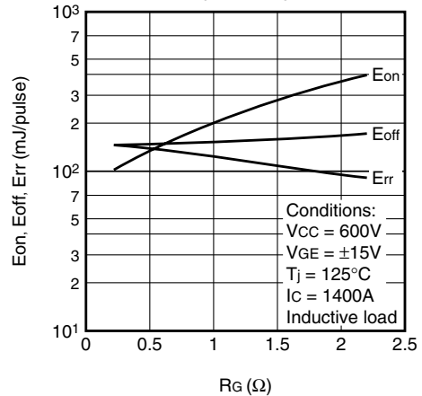
Rg-Esw (TYPICAL)
