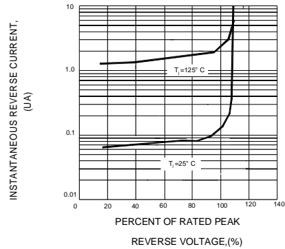
FIG.4-TYPICAL REVERSE CHARACTERISTICS
