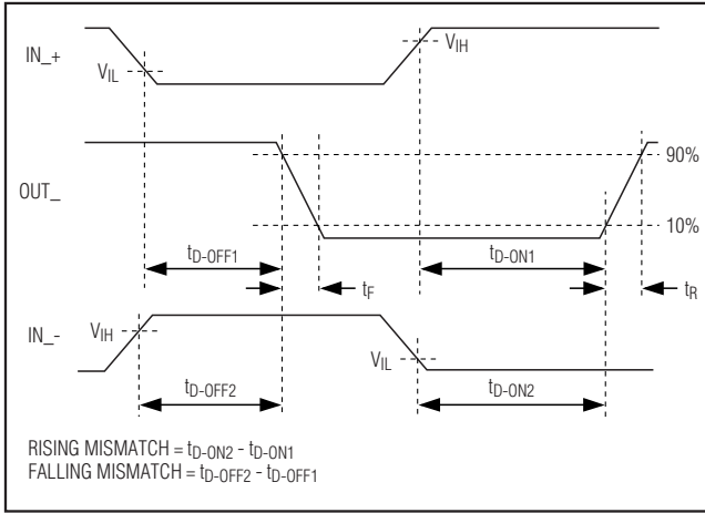
Figure 1. Timing Diagram
