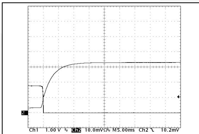
Figure 17: Rise of output voltage after the removal of a short circuit across the output terminals. Ch 1: Vout (1V/div). Ch 2: Iout (20A/div).
