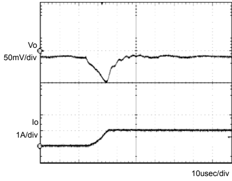
Fig.1 Transient Response (0→1.0A) Co=1 µ F
