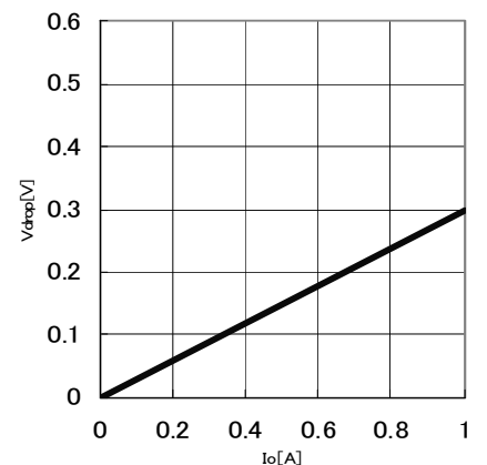
Fig.24 Minimum dropout Voltage 6 (Vcc=12V, Ta=25°C)
