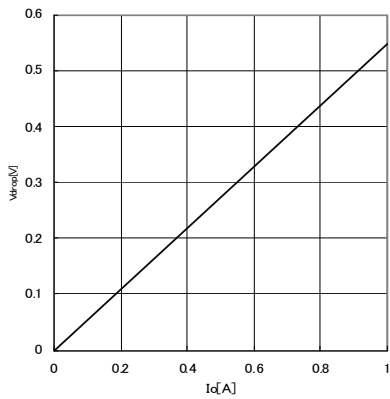
Fig.20 Minimum dropout Voltage 2 (Vcc=4.5V, Ta=25°C)
