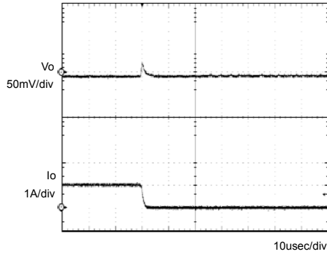
Fig.2 Transient Response (1.0→0A) Co=1 µ F
