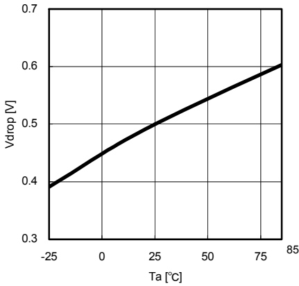
Fig.16 Minimum dropout Voltage 1 (Vcc=5V, Io=-1.0A)
