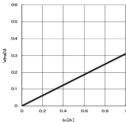
Fig.23 Minimum dropout Voltage 5 (Vcc=10V, Ta=25°C)
