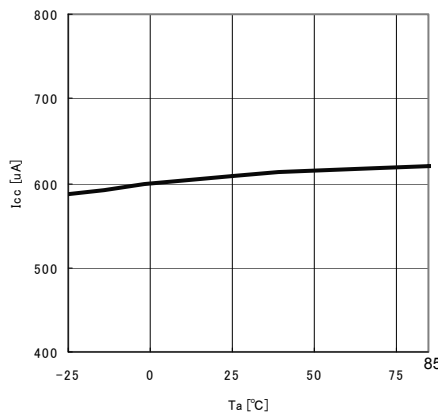
Fig.8 Ta-Icc
