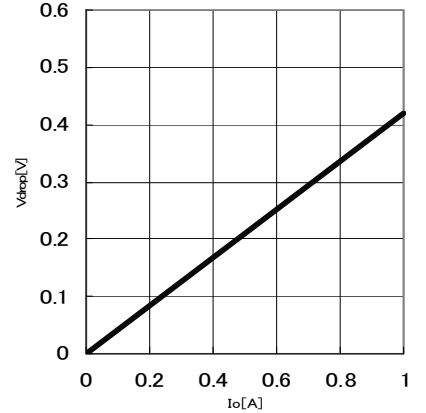
Fig.21 Minimum dropout Voltage 3 (Vcc=6V, Ta=25°C)
