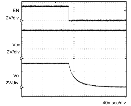
Fig.6 OFF sequence 2 Co=1 µ F
