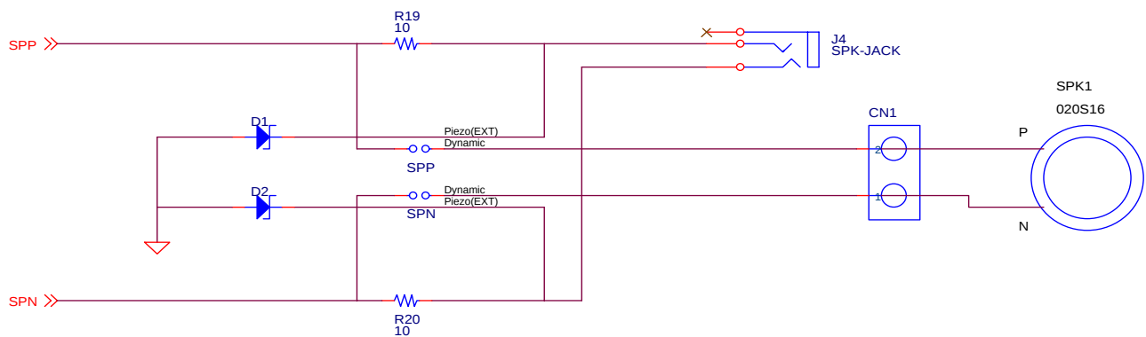
Figure 8. SPEAKER Output Circuit
