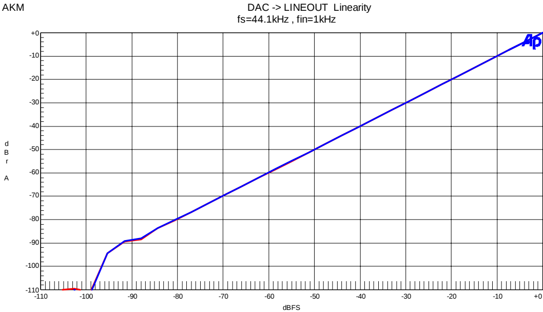
Figure 17. Linearity
