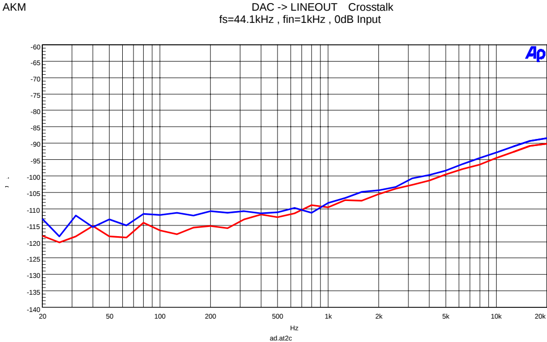
Figure 22. Crosstalk Plot
