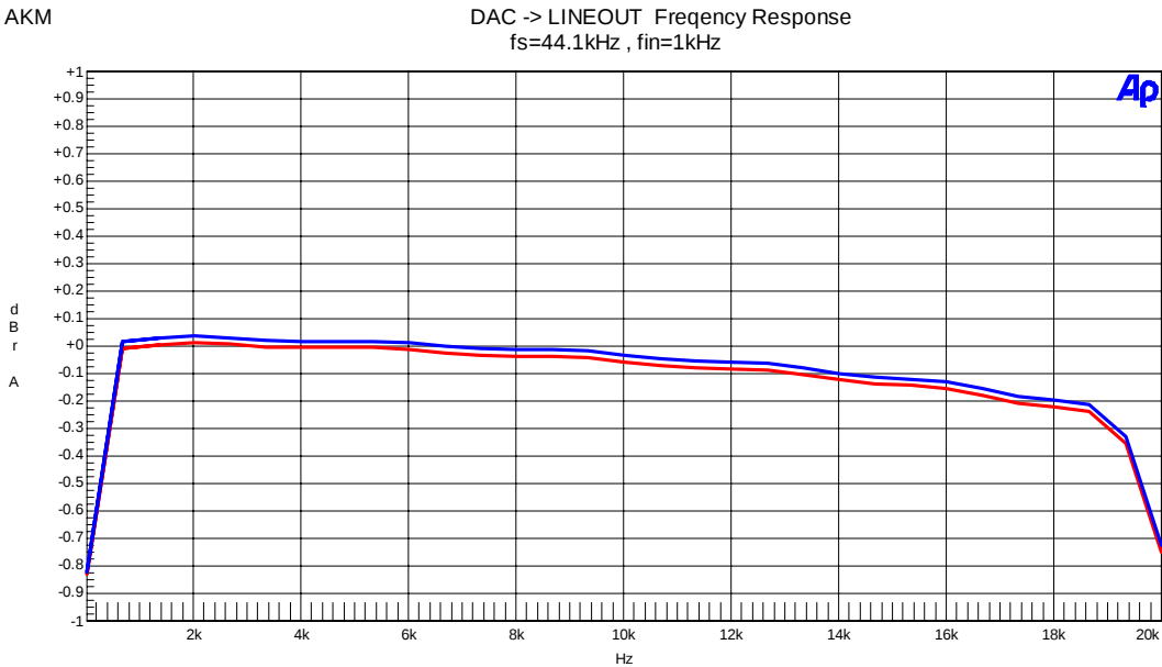
Figure 18. Frequency Response
