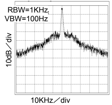
Fig.93 16.9MHz Spectrum VDD=3.3V, at CL=15pF
