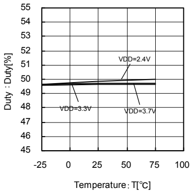
Fig.72 24.6MHz Temperature - Duty
