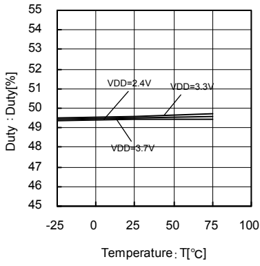
Fig.69 33.9MHz Temperature - Duty
