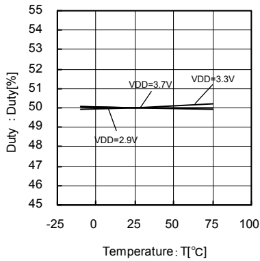
Fig.39 18.4MHz Temperature - Duty
