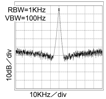
Fig.54 33.9MHz Spectrum VDD=3.3V, at CL=15pF
