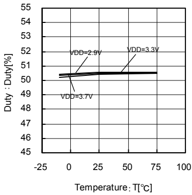
Fig.27 36.9MHz Temperature - Duty
