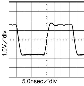
Fig.46 27MHz output waveform VDD=3.3V, at CL=40pF
