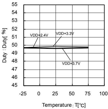
Fig.75 22.6MHz Temperature - Duty
