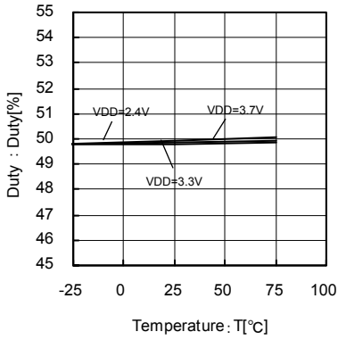
Fig.111 16.9MHz Temperature – Duty
