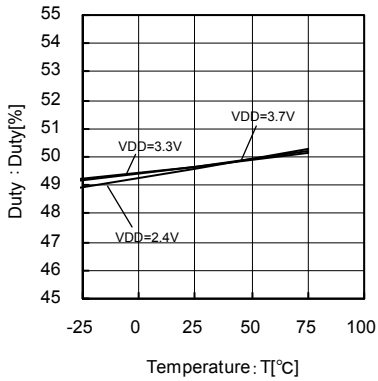
Fig.114 27MHz Temperature – Duty
