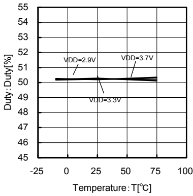
Fig.36 16.9MHz Temperature - Duty
