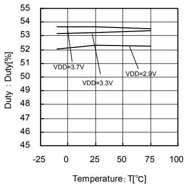
Fig.42 27MHz Temperature - Duty
