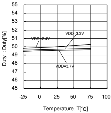
Fig.102 36.9MHz Temperature-Duty
