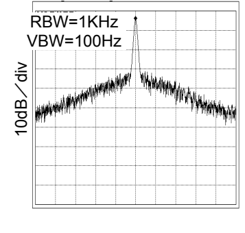
Fig.90 24.6MHz Spectrum VDD=3.3V, at CL=15pF
