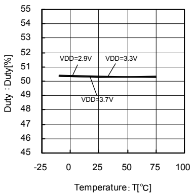
Fig.33 24.6MHz Temperature - Duty
