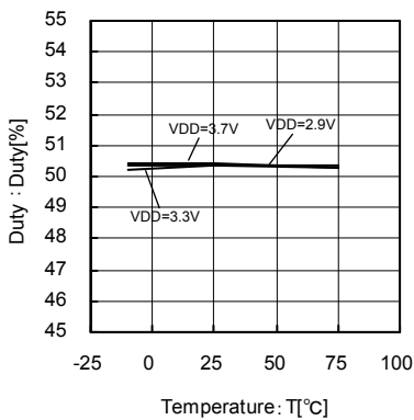
Fig.30 22.6MHz Temperature - Duty
