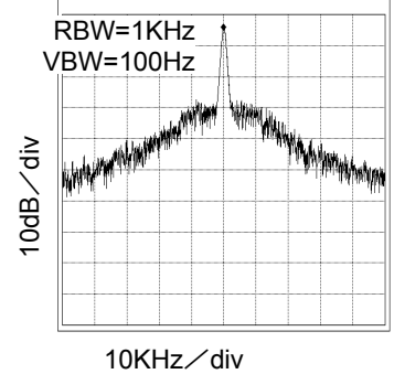
Fig.87 22.6MHz Spectrum VDD=3.3V, at CL=15pF
