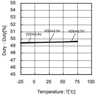
Fig.99 33.9MHz Temperature-Duty
