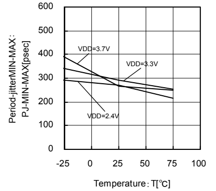
Fig.113 16.9MHz Temperature – Period-Jitter MIN-MAX
