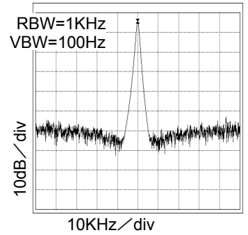
Fig.60 22.6MHz Spectrum VDD=3.3V, at CL=15pF
