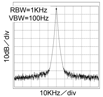
Fig.96 27MHz Spectrum VDD=3.3V, at CL=15pF
