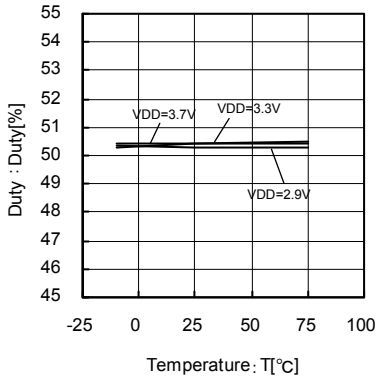
Fig.24 33.9MHz Temperature - Duty
