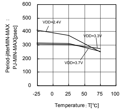
Fig.116 27MHz Temperature – Period-Jitter MIN-MAX
