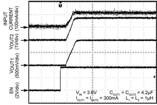
Start-Up Waveform
