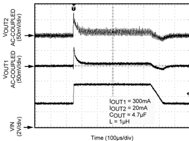
Line Transient
