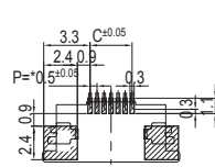
PCB LAYOUT (05003HR-00A02)
