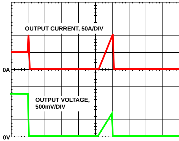
FIGURE 19. OVERCURRENT BEHAVIOR IN HICUP MODE
