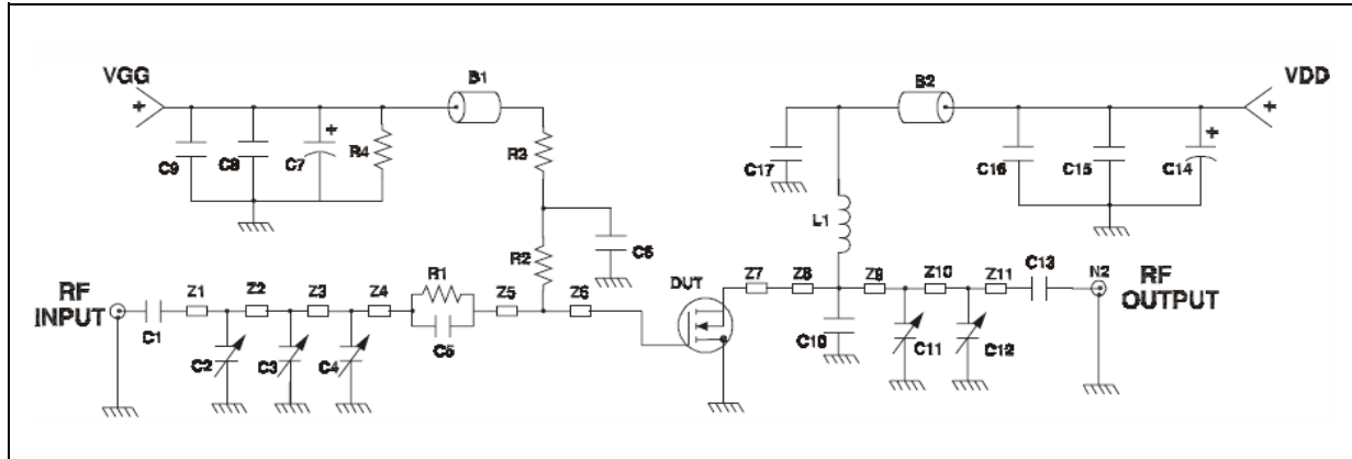
Figure 24. Test circuit schematic
