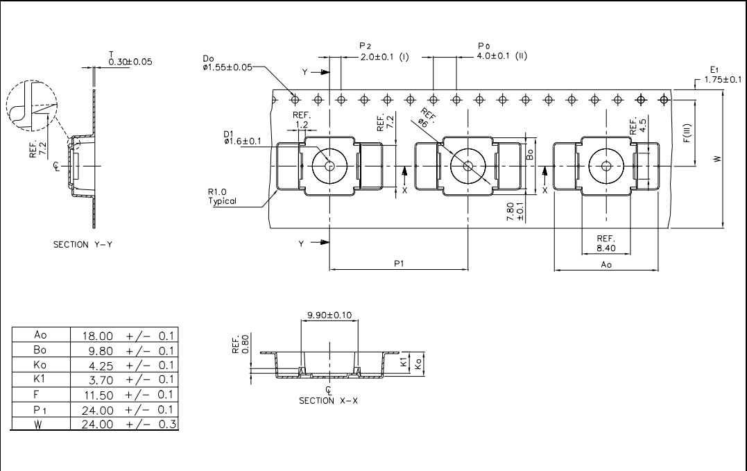
Figure 30. Reel information
