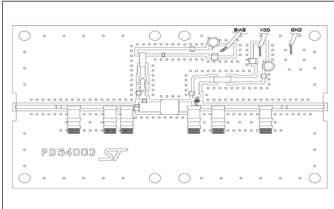
Figure 25. Test fixture component layout
