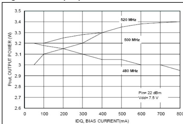
Figure 19. Output power vs. bias current
