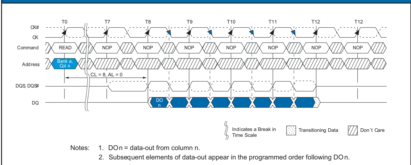
FIGURE 59 - READ LATENCY
