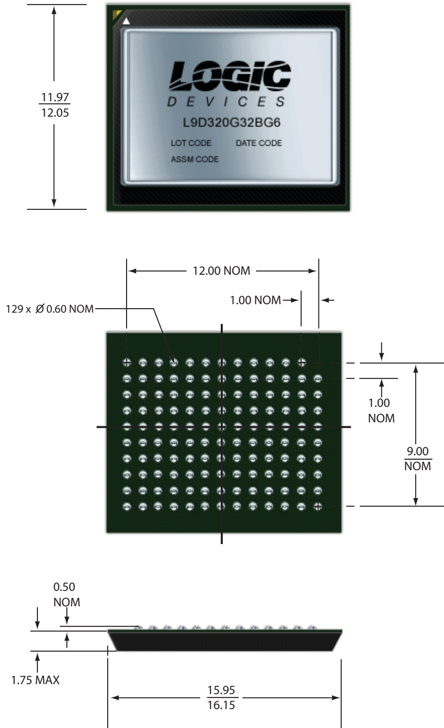
FIGURE 5 - MECHANICAL DRAWING
