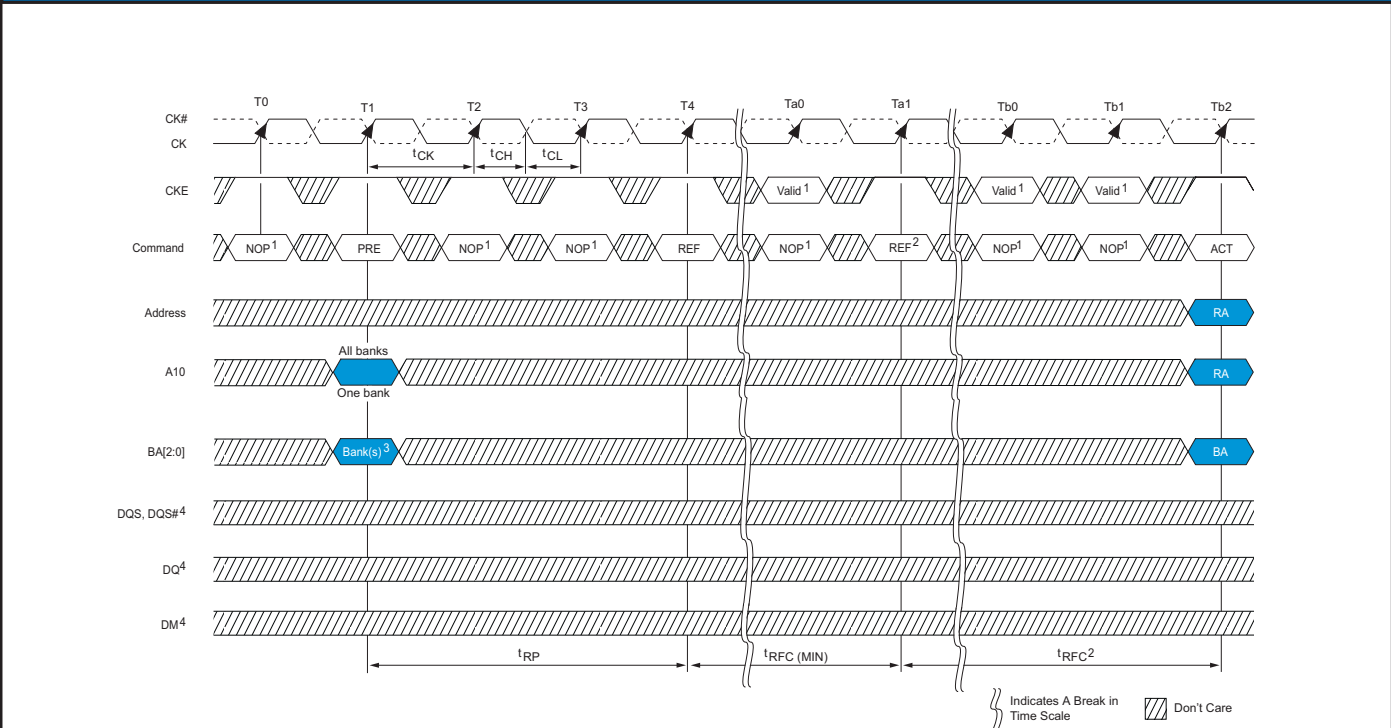
FIGURE 33 - REFRESH MODE
