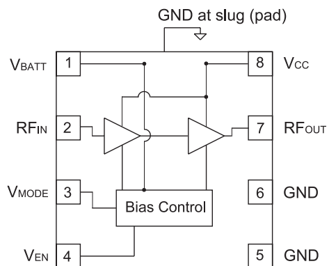
Figure 1: Block Diagram
