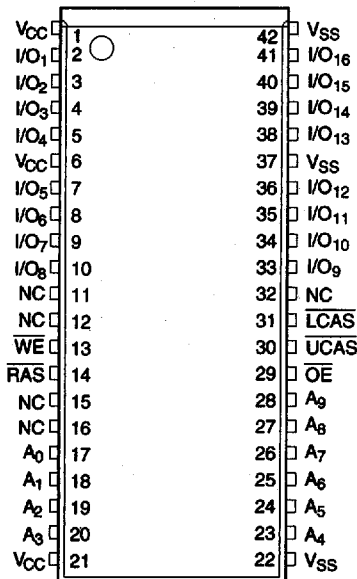
42-pin SOJ (400mil) P42SJ-2B-L
