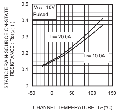
Fig.6 Static Drain-Source On-State Resistance vs. Channel Temperature
