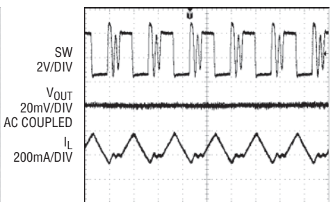
Discontinuous Operation
