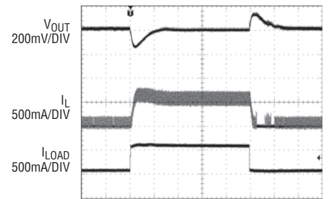
Load Step
