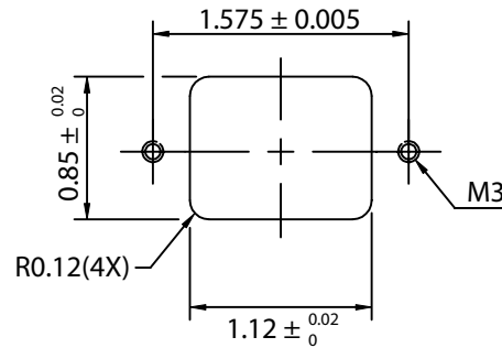
PANEL CUTOUT (MOUNTING FROM FRONT)
