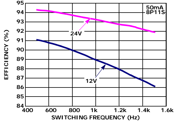
FIGURE 6. EFFICIENCY vs SWITCHING FREQUENCY
