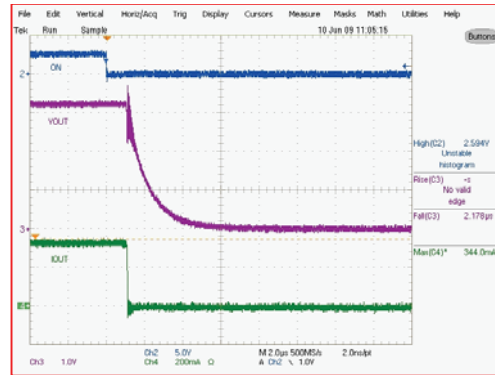
Figure 25. Turn-Off Response (V_{IN}=3.3V, C_{IN}=1\mu F, C_{OUT}=0.1\mu F, R_L=100\Omega)
