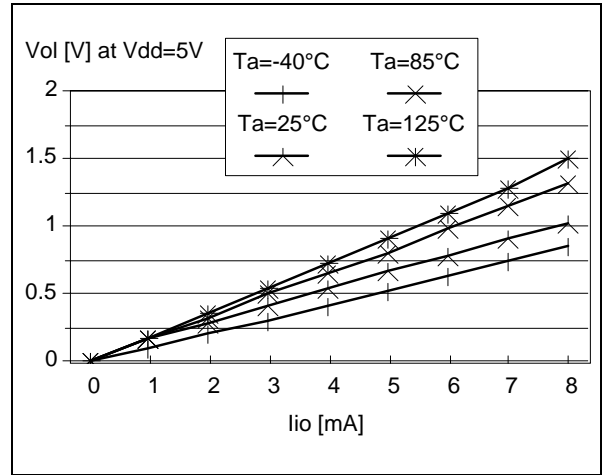
Figure 87. Typical V_{OL} at V_{DD}=5V (RESET)
