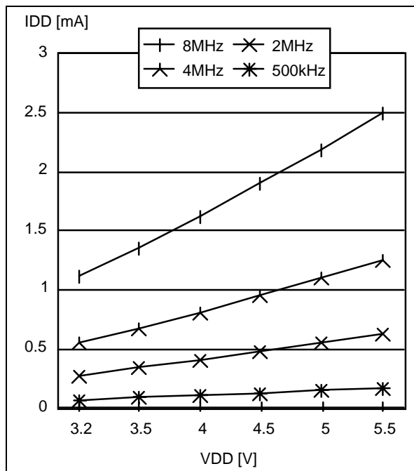
Figure 60. Typical I DD in WAIT vs. f CPU
