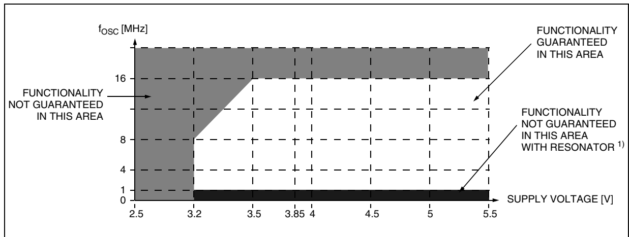
Figure 50. f_{OSC} Maximum Operating Frequency Versus V_{DD} Supply Voltage for ROM Devices 2)
