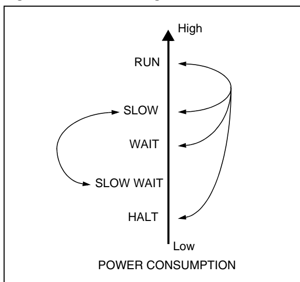
Figure 15. Power Saving Mode Transitions
