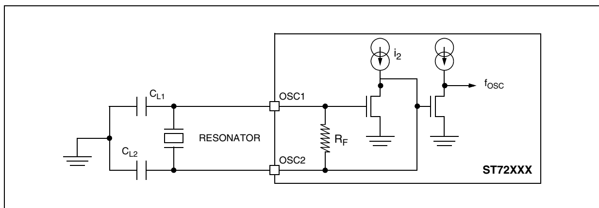
Figure 63. Typical Application with a Crystal Resonator
