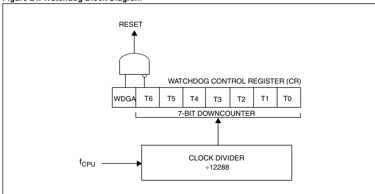
Figure 24. Watchdog Block Diagram
