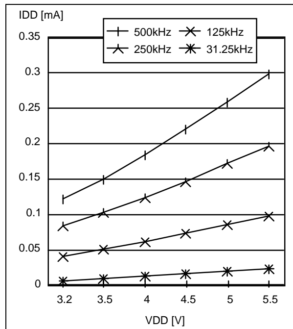
Figure 61. Typical I DD in SLOW-WAIT vs. f CPU
