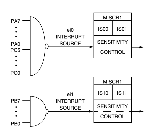
Figure 23. Ext. Interrupt Sensitivity (EXTIT=1)
