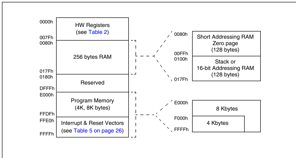
Figure 3. Memory Map
