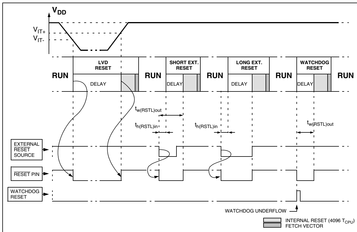
Figure 11. RESET Sequences
