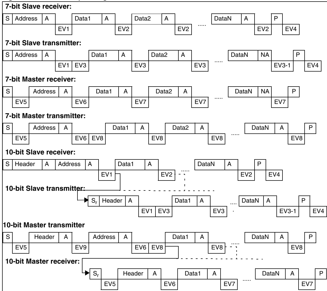
Figure 44. Transfer Sequencing
