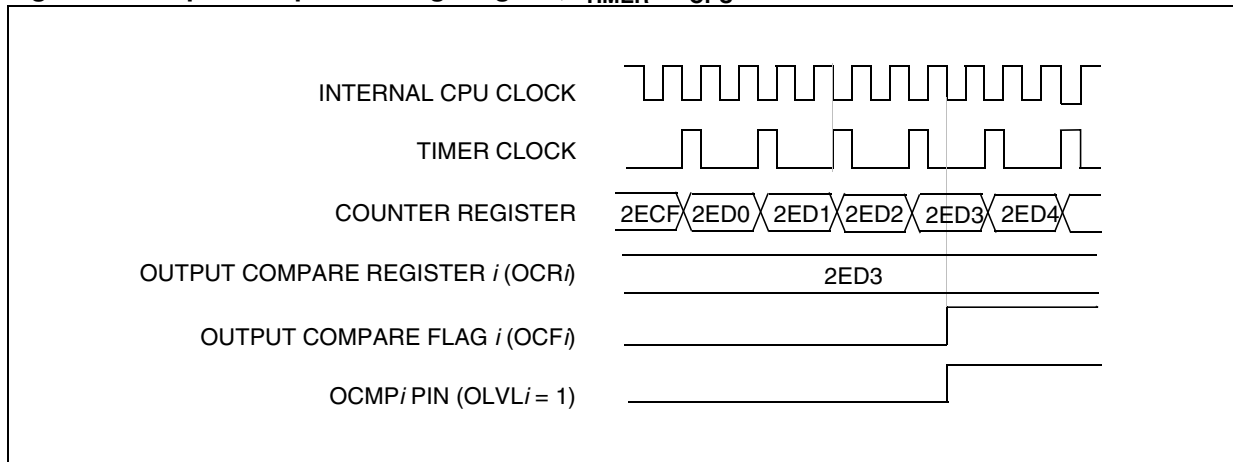
Figure 32. Output Compare Timing Diagram, f_{\text{TIMER}} = f_{\text{CPU}}/2
