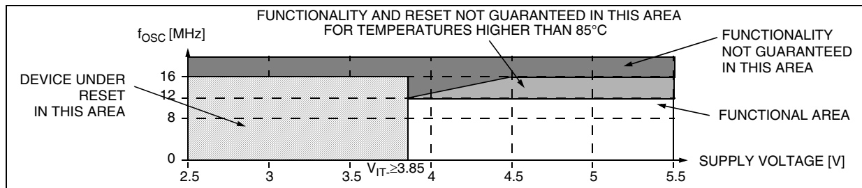
Figure 53. Medium LVD Threshold Versus V_{DD} and f_{OSC} for Flash devices 3)
