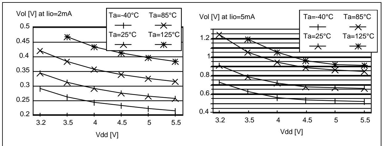
Figure 88. Typical V_{OL} vs. V_{DD} (RESET)
