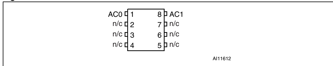
Figure 2. MLP connections
