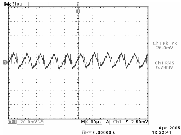
24 Vdc input, 3.3 Vdc/15 A output
