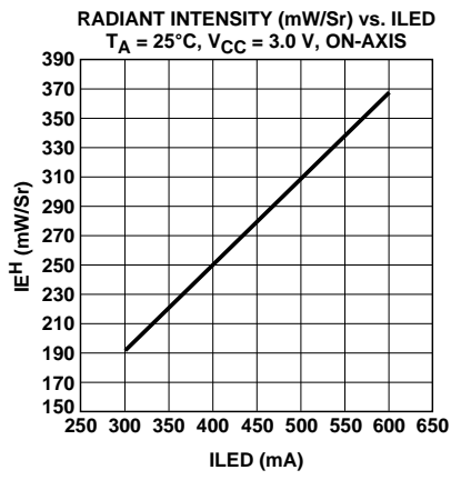
Figure 5. IR LOP vs. ILED.
