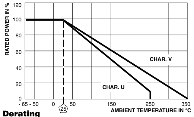
Derating
