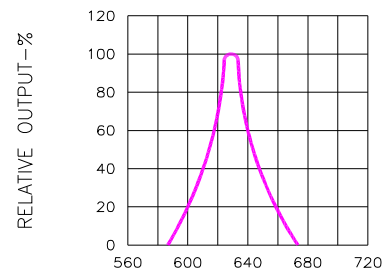
Fig.2 SPECTRAL RESPONSE
