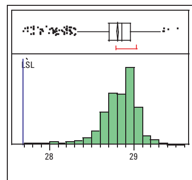
P-1dB at 28 GHz
