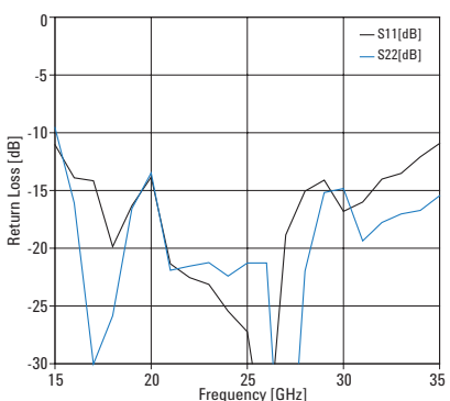
Figure 2. Typical Return Loss (Input and Output)
