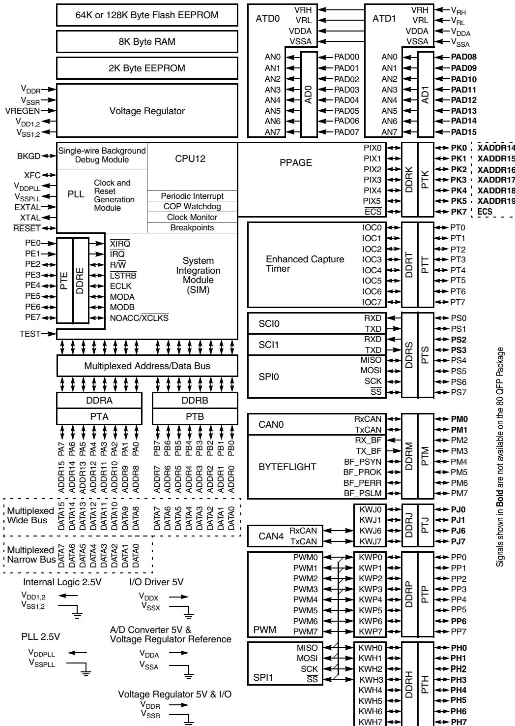
Figure 1. MC9S12DB Family Block Diagram
