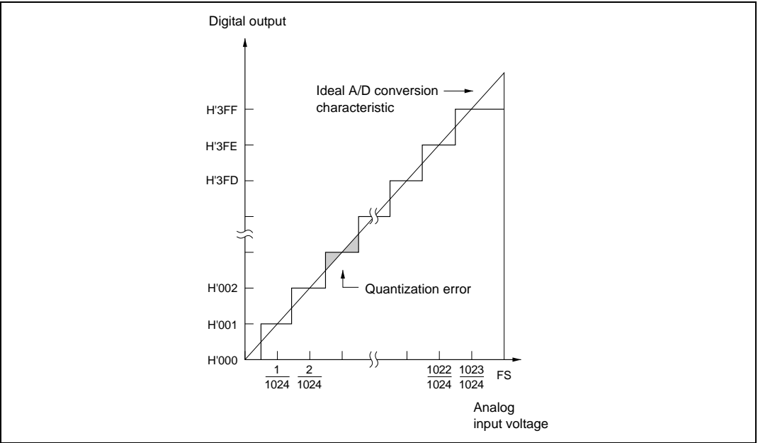
Figure 14.9 A/D Conversion Precision Definitions (1)
