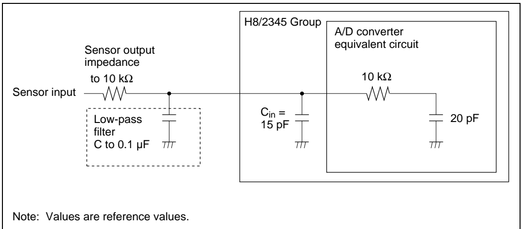
Figure 14.11 Example of Analog Input Circuit
