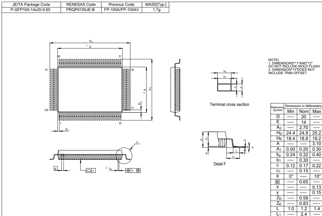
Figure G.3 FP-100A Package Dimensions
