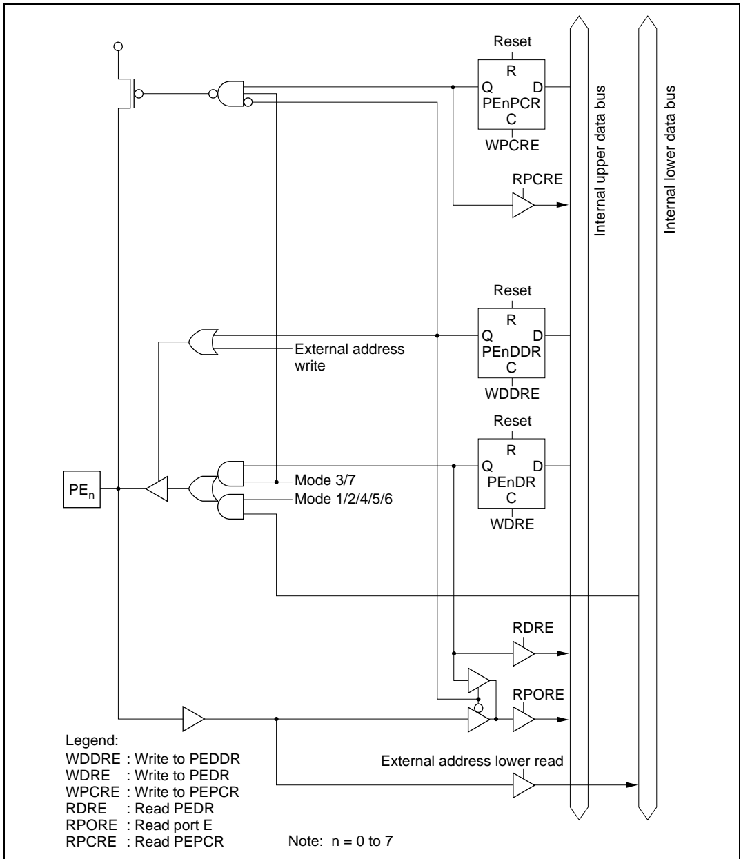
Figure C.9 Port E Block Diagram (Pin PE_n )
