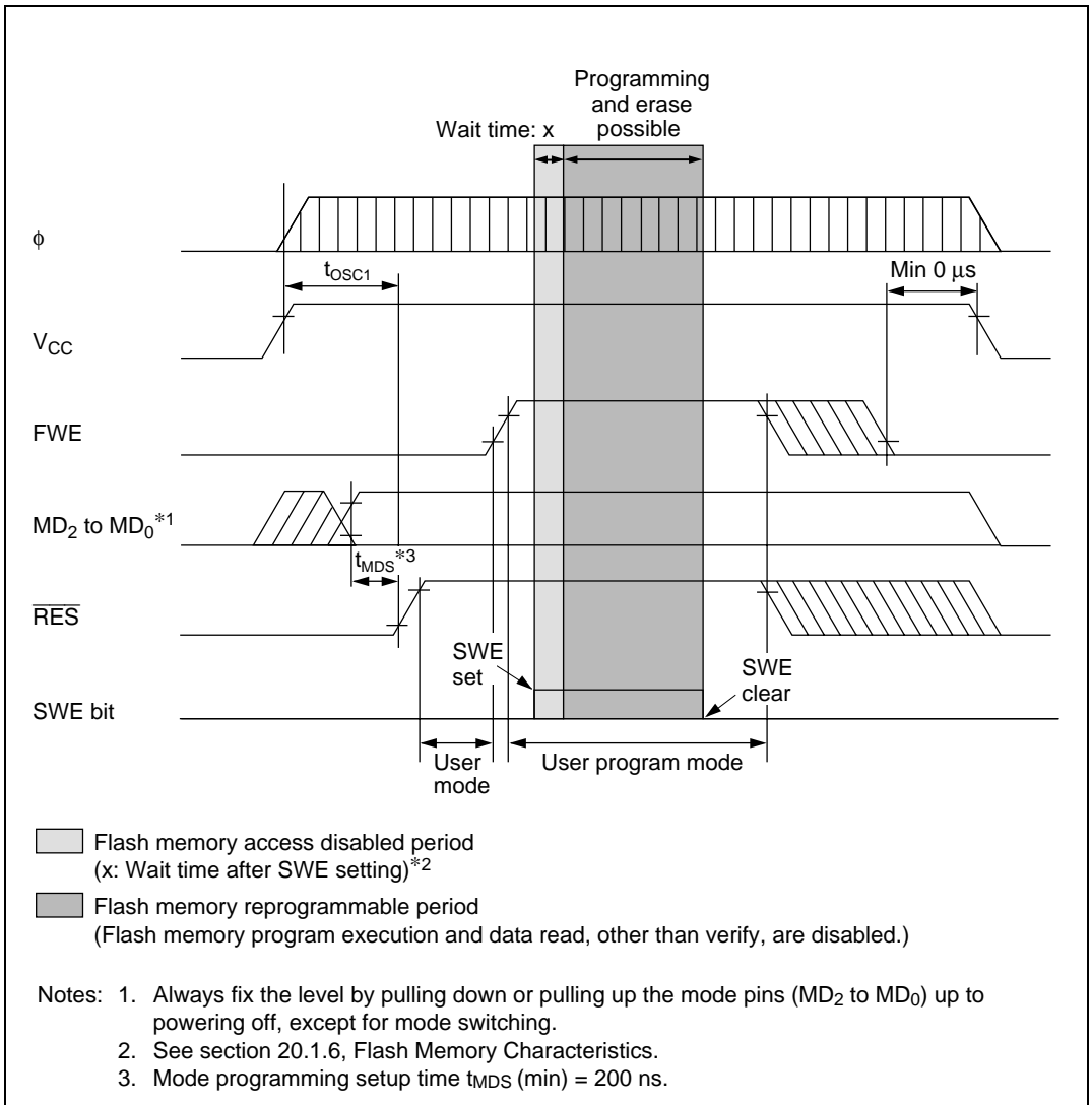
Figure 17.37 Powering On/Off Timing (User Program Mode)
