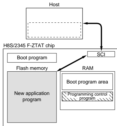
Figure 17.9 Boot Mode
