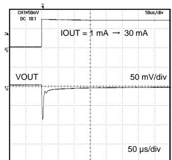
Fig. 20 Load Response (Co = 1.0 µF) (BH33RB1WGUT)
