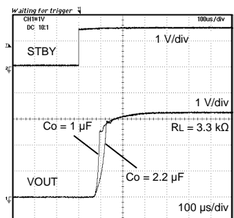
Fig. 23 Output Voltage Rise Time (BH33RB1WGUT)
