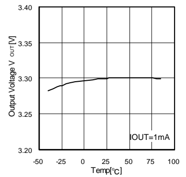
Fig. 14 Output Voltage vs Temperature (BH33RB1WGUT)
