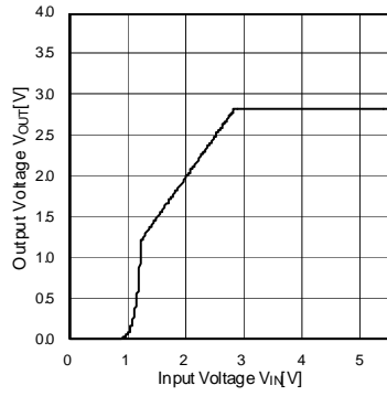
Fig. 2 Output Voltage vs Input Voltage (BH28RB1WGUT)
