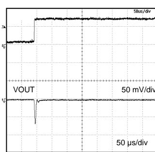
Fig. 19 Load Response (Co = 1.0 µF) (BH28RB1WGUT)
