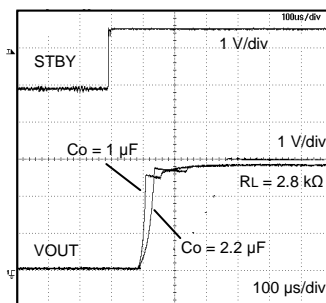
Fig. 22 Output Voltage Rise Time (BH28RB1WGUT)
