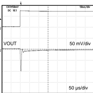
Fig. 18 Load Response (Co = 1.0 µF) (BH15RB1WGUT)
