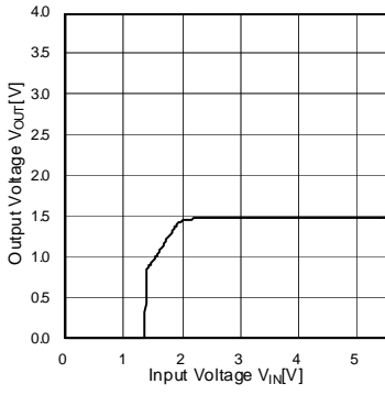
Fig. 1 Output Voltage vs Input Voltage (BH15RB1WGUT)
