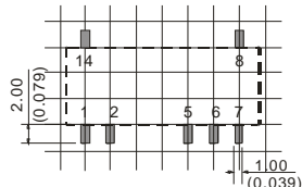
FOOTPRINT DETAILS
