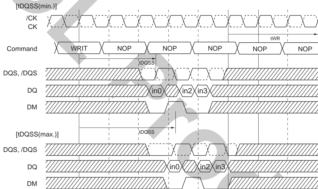
Data Mask Function, WL = 3, AL = 0 shown
