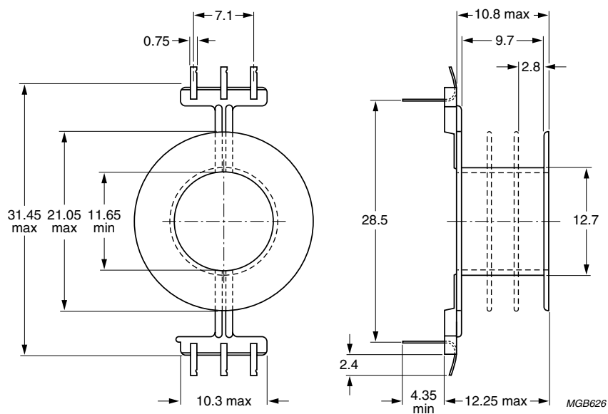
Fig.4 P26/16 coil former for PCB mounting; 6-pins.
