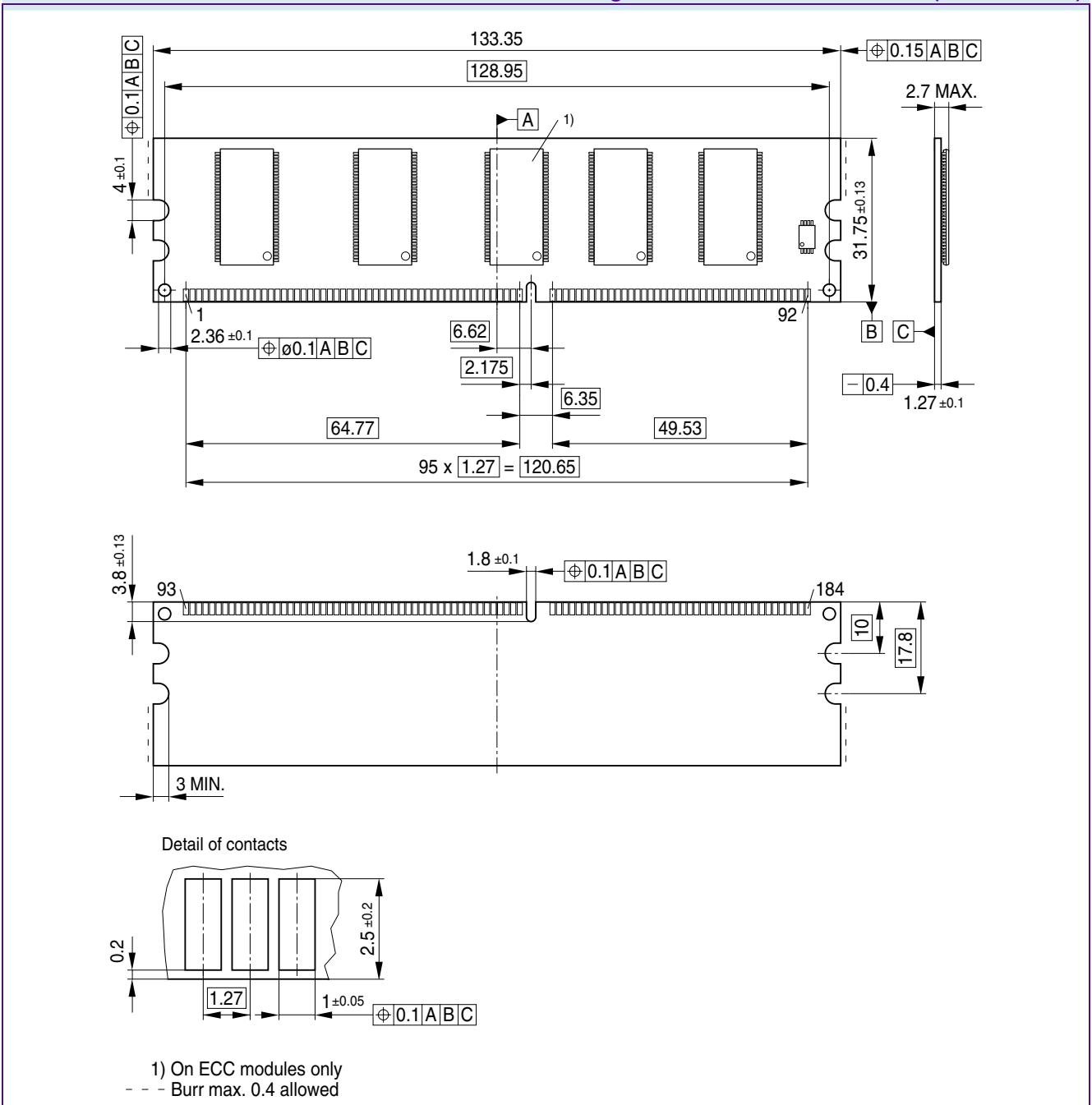
FIGURE 8 Package Outline UDIMM Raw Card C (L-DIM-184-18)
