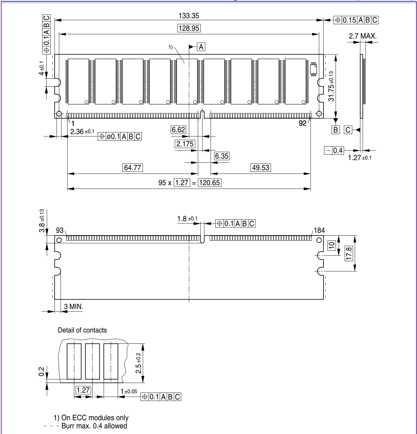
FIGURE 10 Package Outline UDIMM Raw Card A (L-DIM-184-30)
